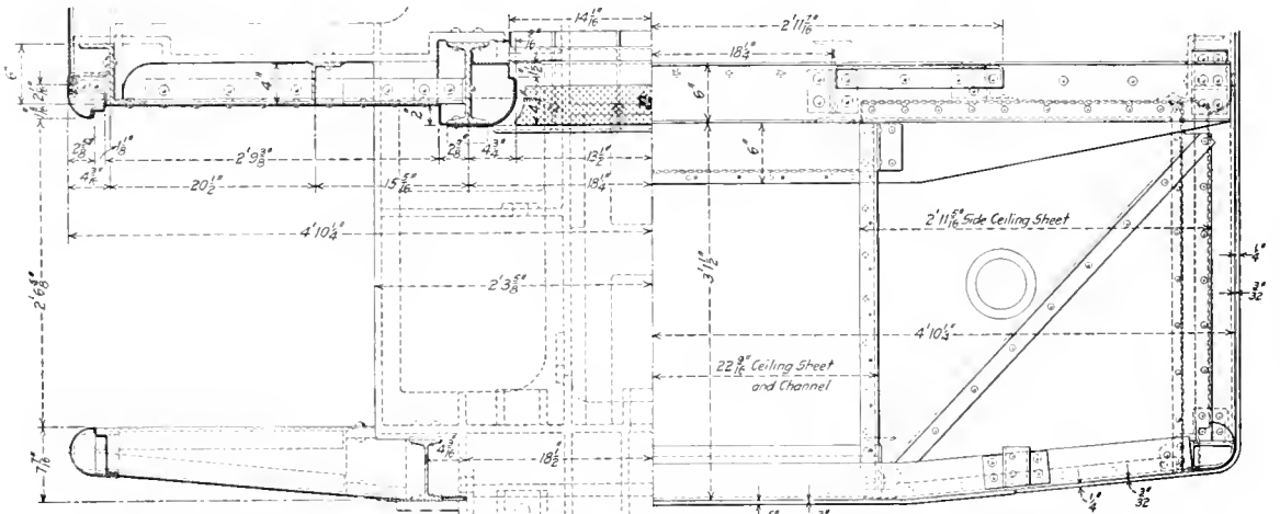
Side Framing of the D. & H. Coaches
